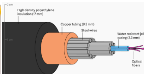
Fiber Optic
